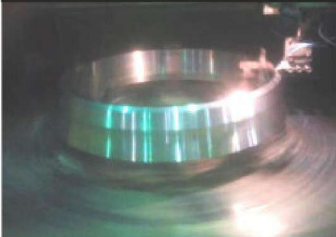
TORICON PROFILE MACHINING ON CNC VTL
